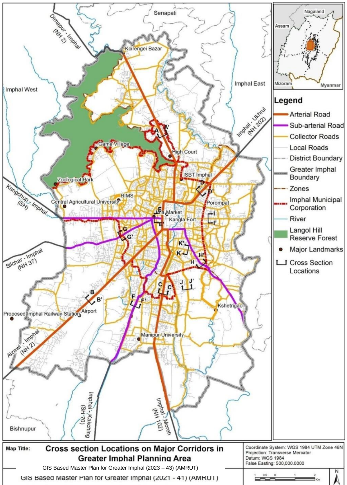
Map 8. 4: Cross Section Locations on Major Corridors in Greater Imphal Planning Area
