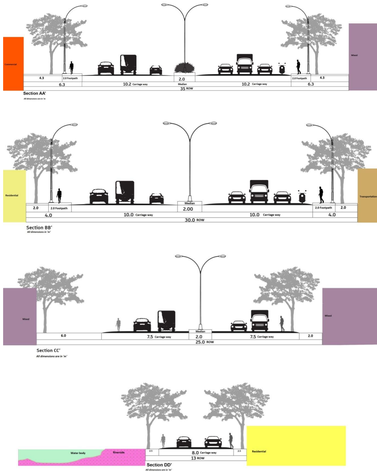
Figure 8. 1: Selected arterial road cross sections in Greater Imphal Planning Area
